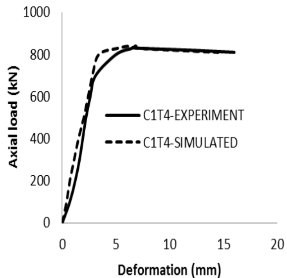
Fig.5. Experiment Vs. simulated load-deformation curve for C1T4 column
