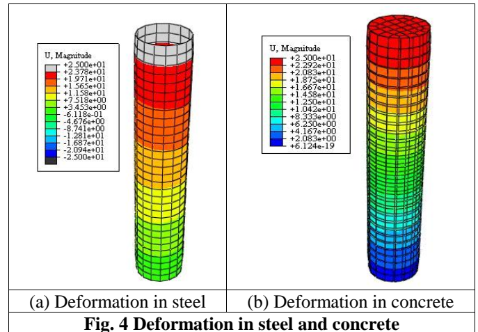
Fig. 4 Deformation in steel and concrete
