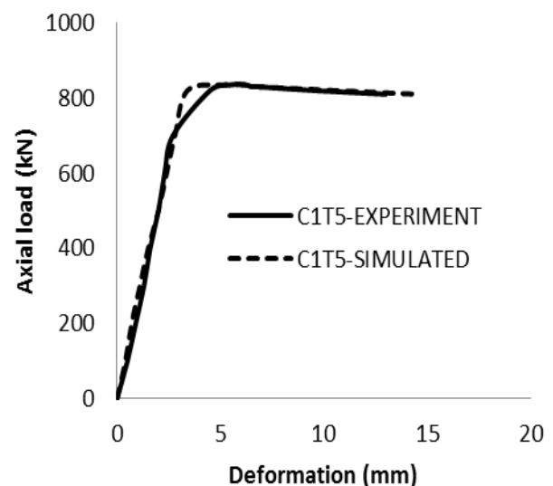
Fig.6. Experiment Vs. simulated load-deformation curve for C1T5 column
