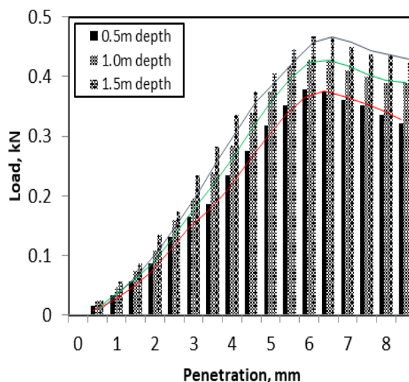
Fig. 8(b) Histogram of Load and Penetration for contaminated soil (soaked condition).
