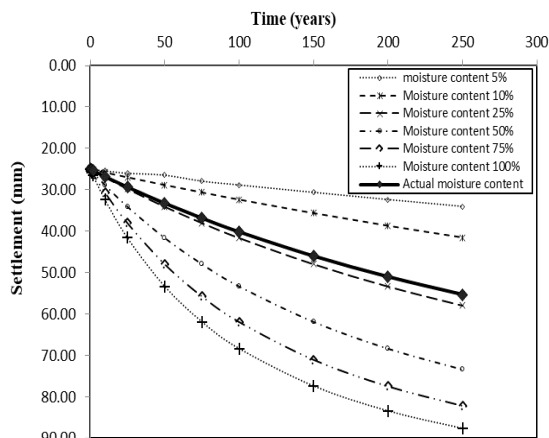
Fig. 11. Settlement of soil with variation in moisture content.
