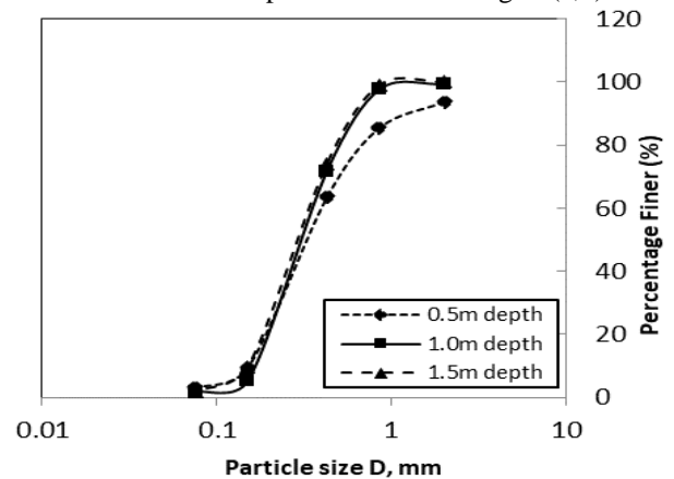
Fig. 4(a) Particle Size Distributions for contaminated soil.
