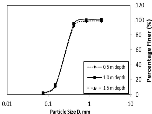
Fig. 4(b) Particle Size Distributions for un-contaminated soil.
