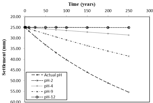
Fig. 10. Settlement of soil with variation in pH for biodegradation model.
