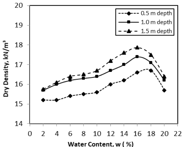
Fig. 5(a) Compaction Curve of contaminated soil from Standard Proctor Test.
