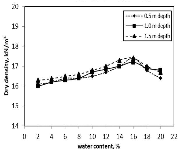
Fig. 5(b) Compaction Curve of uncontaminated soil from Standard Proctor Test.
