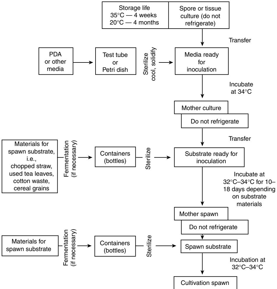
FIGURE 14.9 Spawn production flowchart for V. voluacea .
