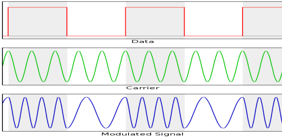
Fig 3.1: FSK waveforms
