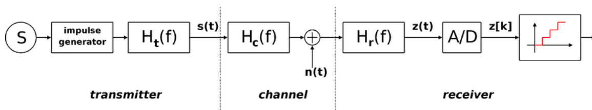
Fig 2.1: Block diagram of ASK Source : en.wikipedia.org/wiki/Amplitude-shift_keying
