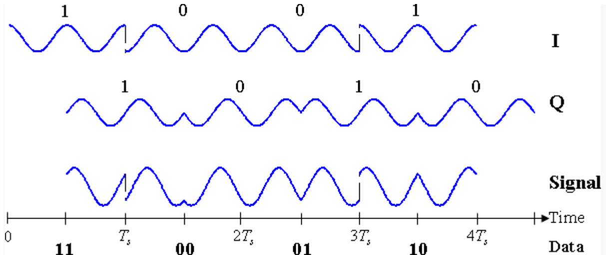
Fig 4.14: Timing diagram for offset-QPSK.
