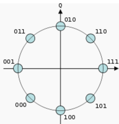
Fig 4.17: Constellation diagram for 8-PSK with Gray coding.
