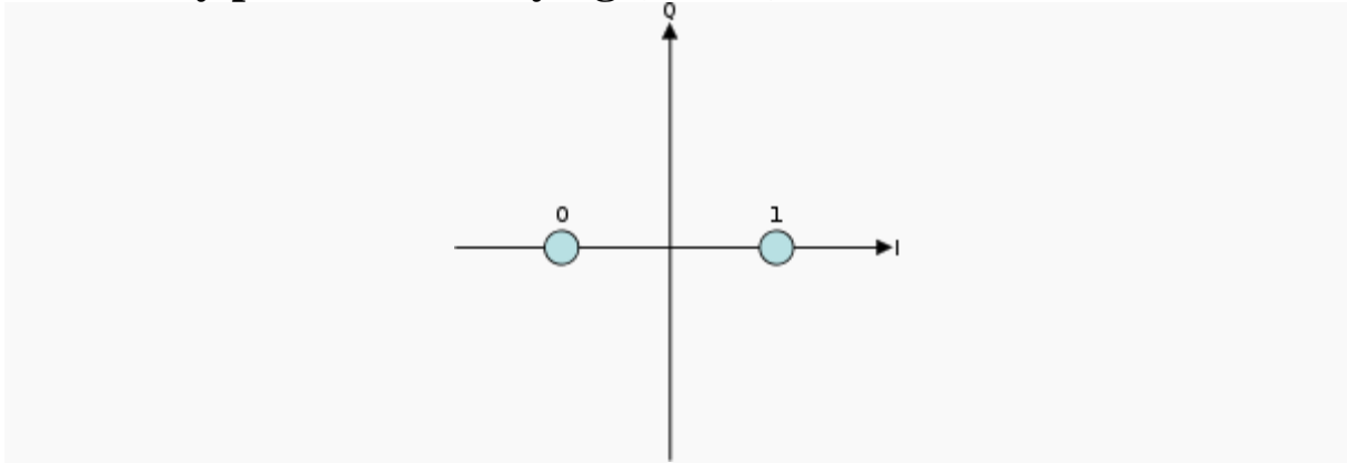
Fig 4.2: Constellation diagram of BPSK
