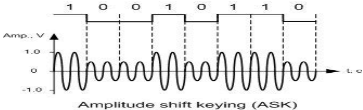
Fig 2.2: A BASK modulated signal (lower), together with its input bit stream.
