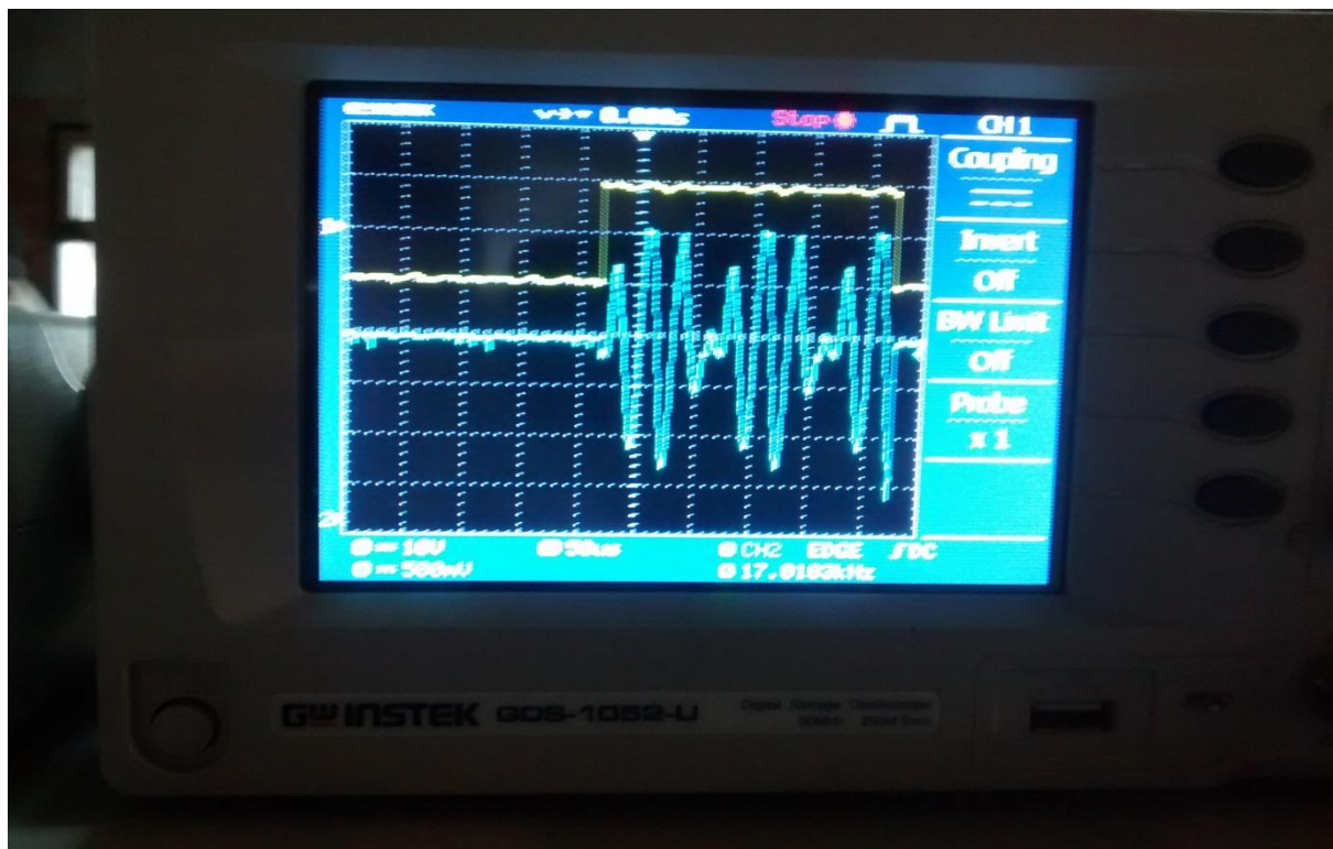
FSK waveform
