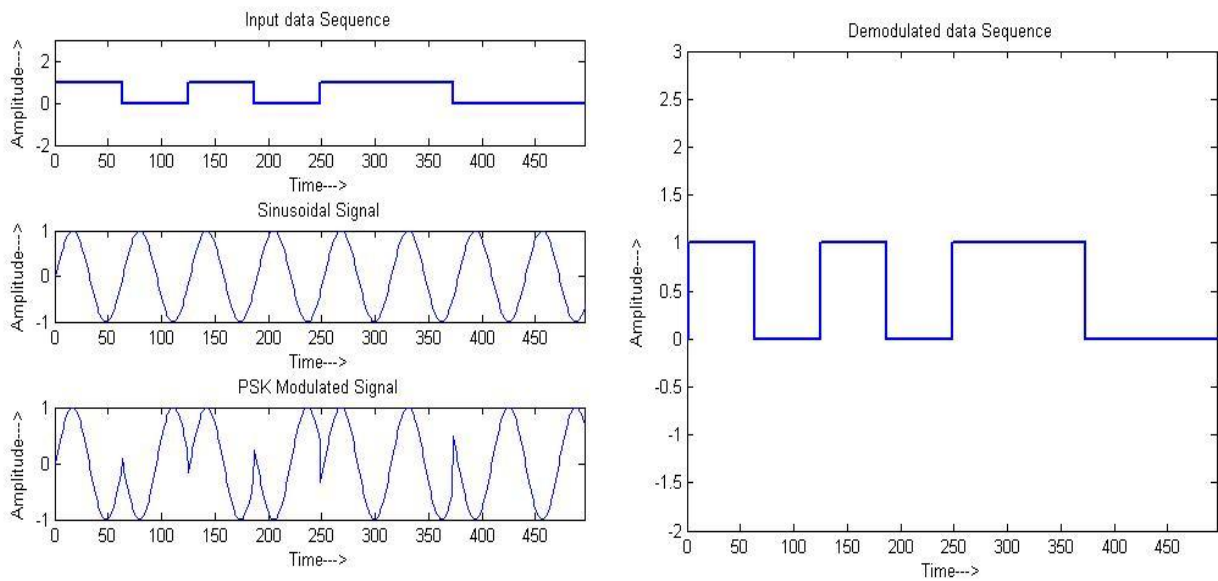
Fig 4.1: Input, carrier and modulated wave and demodulated wave.
