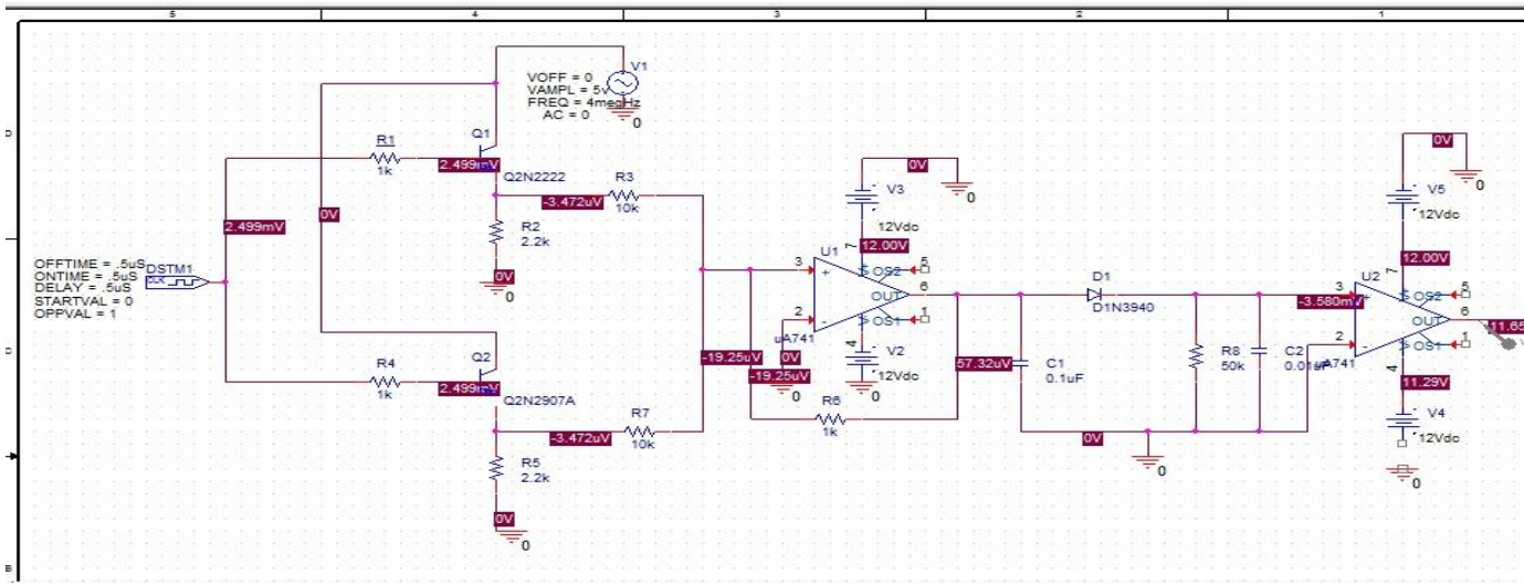
Fig 3.2: circuit diagram of FSK modulation and demodulation.
