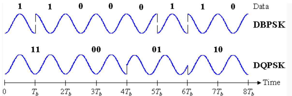
Fig 4.18: Timing diagram for DBPSK and DQPSK.
