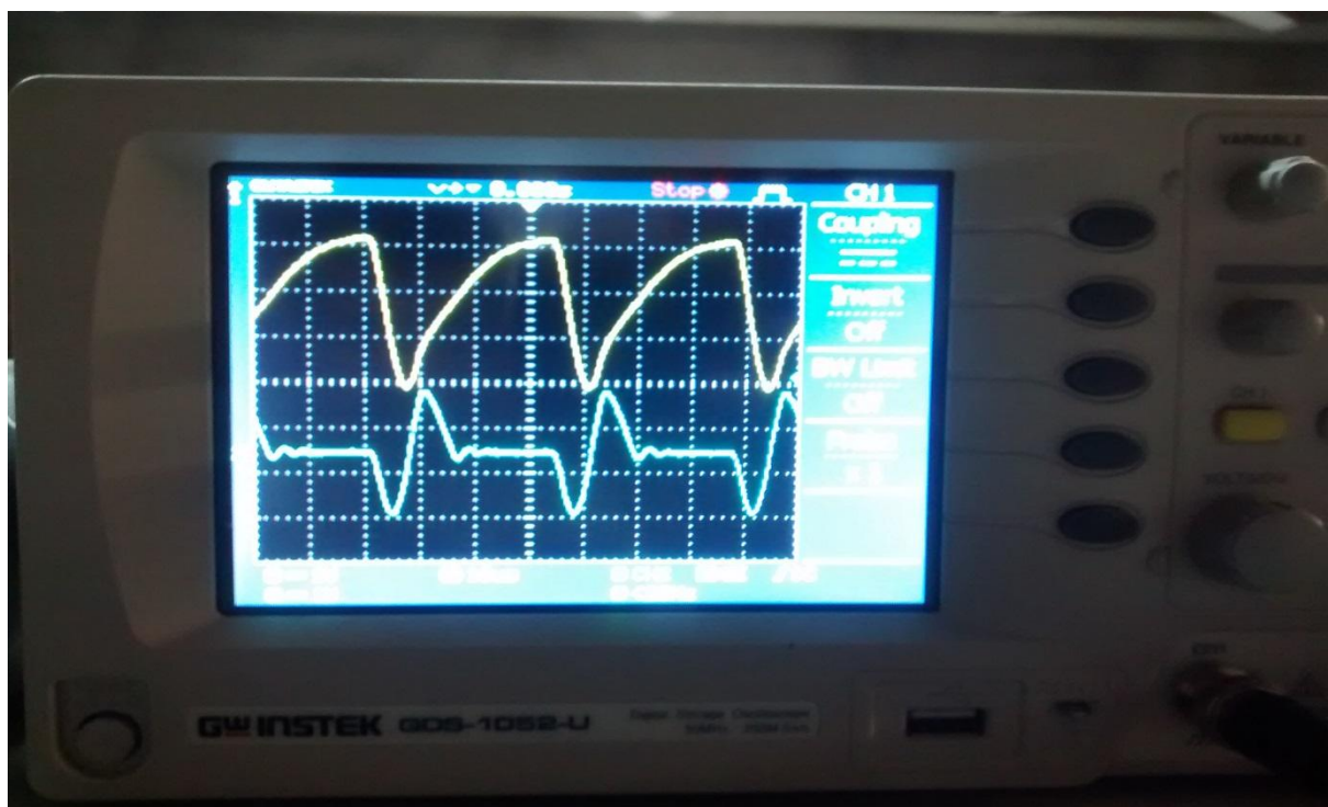
PSK waveform
