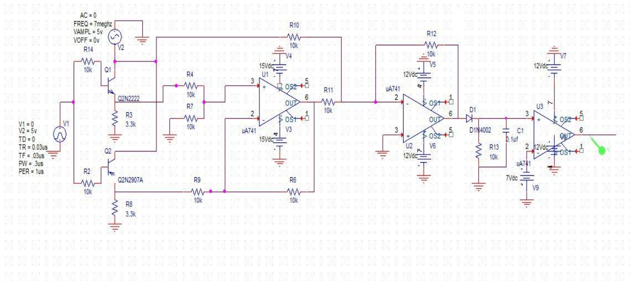
Fig 4.19: Circuit diagram modulation and demodulation
