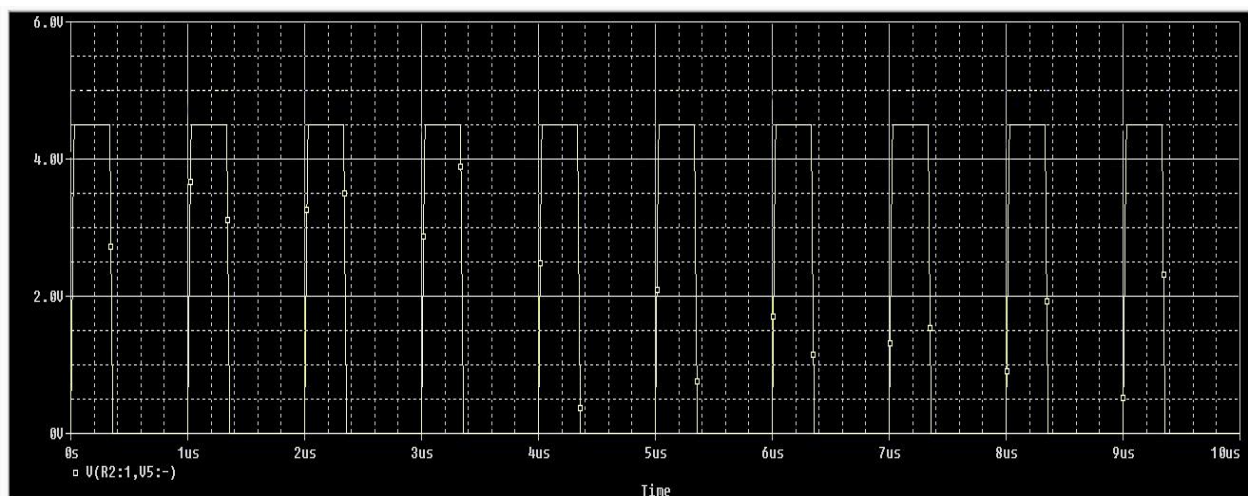
Fig 4.20: Resultant waveform after demodulation
