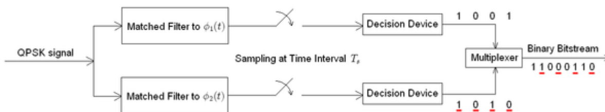
Fig 4.10: Block diagram of QPSK
