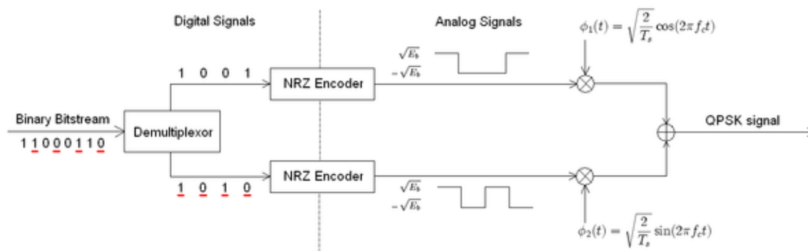
Fig 4.9: Conceptual transmitter structure for QPSK.
