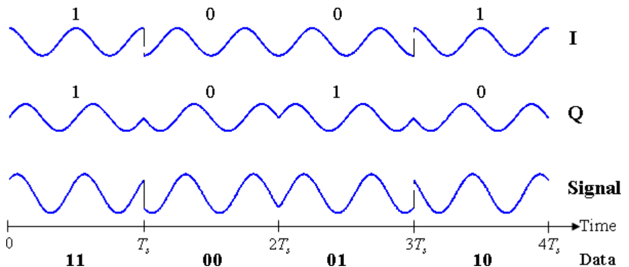
Fig 4.11: Timing diagram for QPSK
