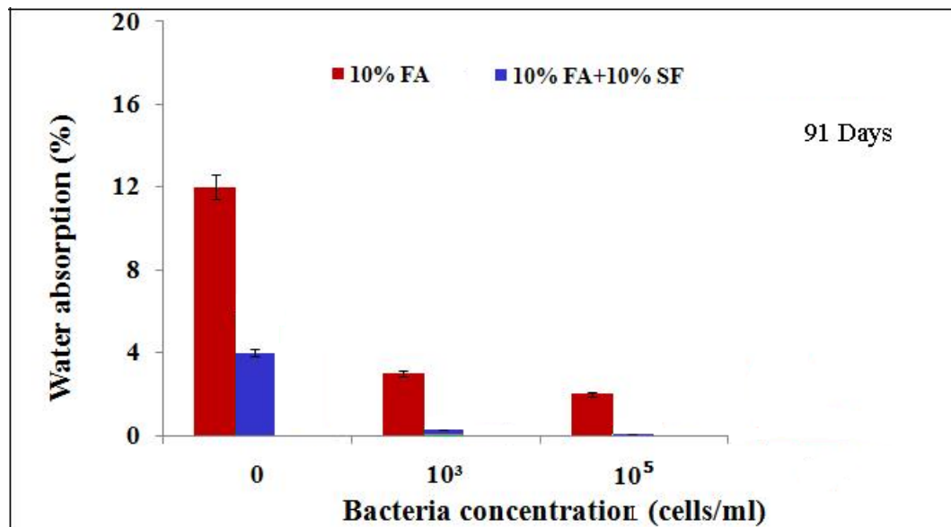
Figure 4.5: Effect of Bacteria on Water Absorption of (10%) Fly Ash and (10%) Silica Fume Concrete.
