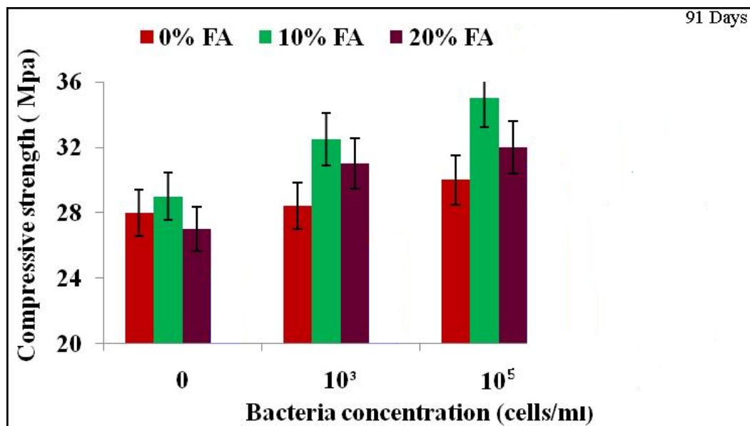
Figure 4.2: Effect of Bacteria on Compressive Strength of Concrete
