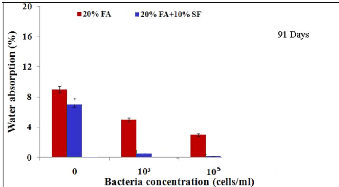
Figure 4.6: Effect of Bacteria on Water Absorption of (20%) Fly Ash and (10%) Silica Fume Concrete.
