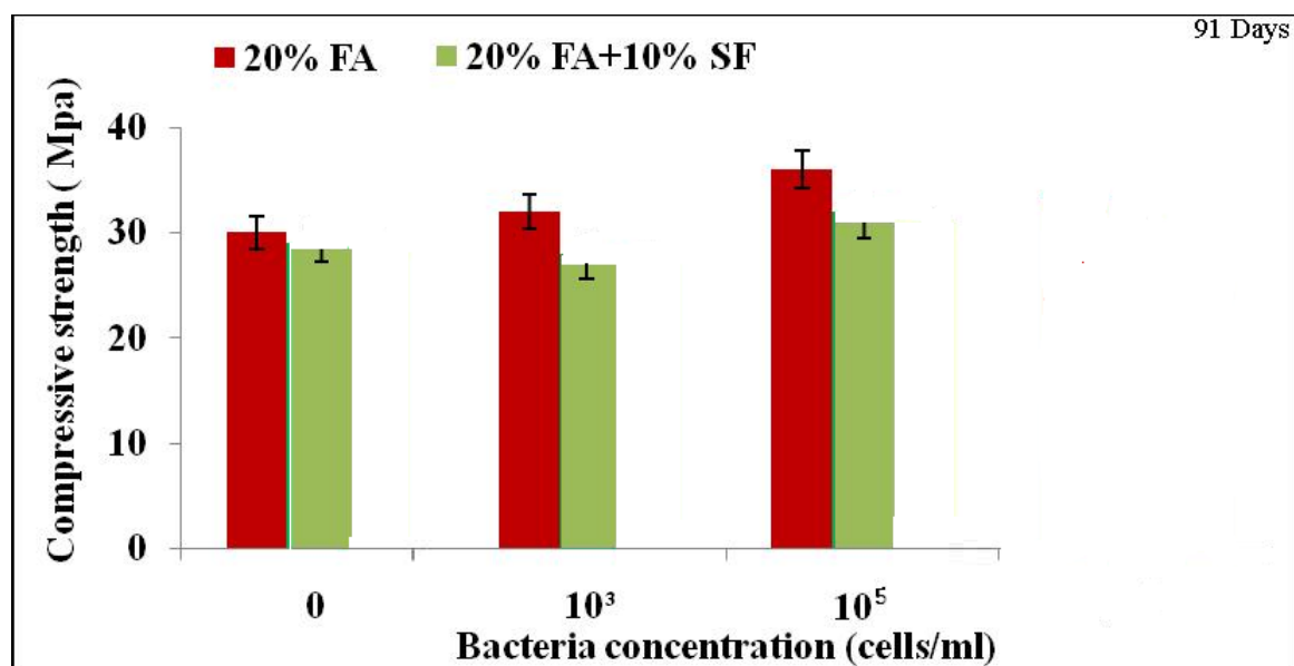
Figure 4.3: Effect of Bacteria on Compressive Strength of (10,20%) Fly Ash and (10%) Silica Fume Concrete
